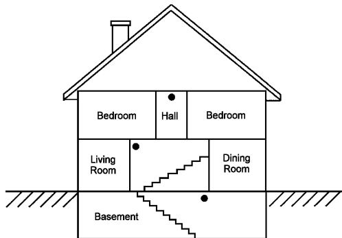
Figure 2: IN FAMILY LIVING UNITS WITH MORE THAN ONE SLEEPING AREA, A SMOKE ALARM SHOULD BE PROVIDED TO PROTECT EACH SLEEPING AREA IN ADDITION TO ALARMS REQUIRED IN BEDROOMS.
